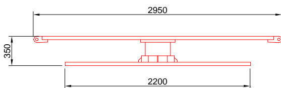
SIDE ELEVATION BOLSTER WITHOUT SLIPPER
