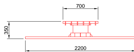
END ELEVATION BOLSTER WITHOUT SLIPPER
