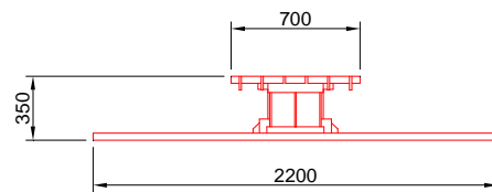
END ELEVATION BOLSTER WITH SLIPPER
