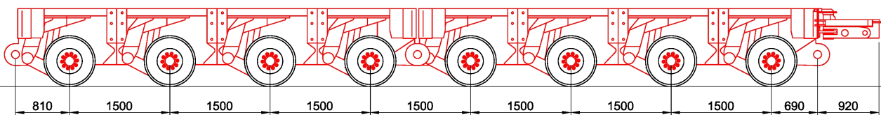
SIDE ELEVATION
