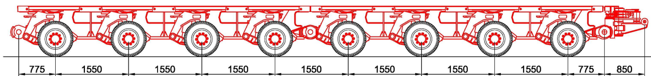
SIDE ELEVATION
